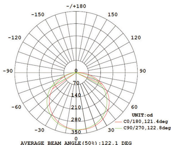
Photometric of 1M strip
