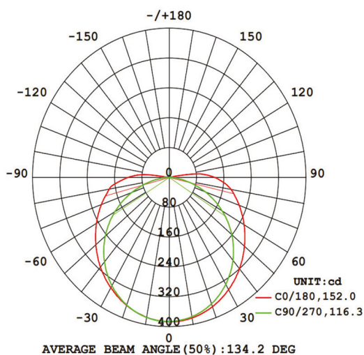
Photometric of 1M (4000K) strip
